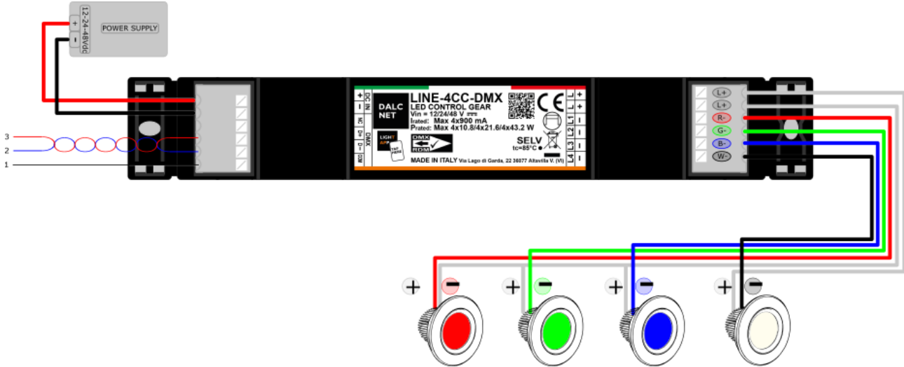
Figure 5: Wiring diagram for RGBW LED load
