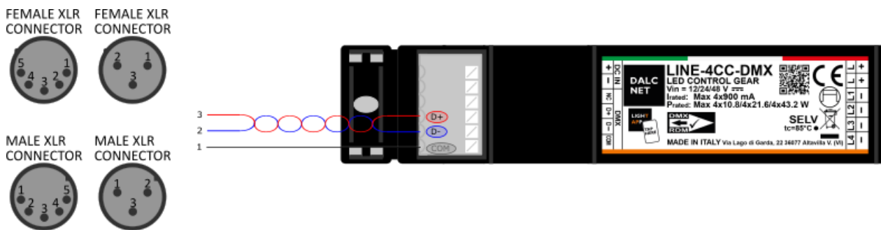
Figure 6: Remote Control connection pin-out and XLR connectors
